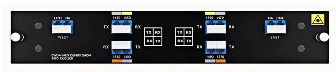
2CH CWDM OADM Single Fiber
