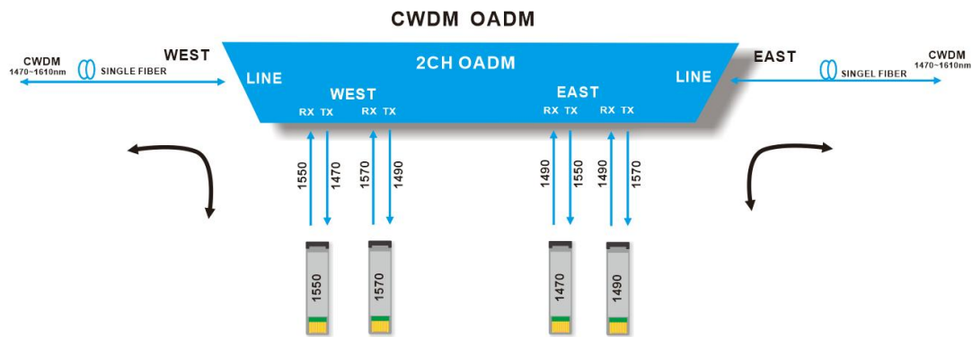
2CH CWDM Single fiber transmission
