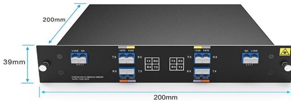
Plug-in LGX Box
