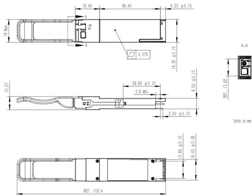
Figure2. Mechanical Outline
