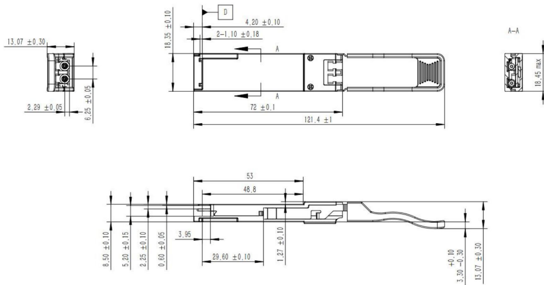
Figure 2. Mechanical dimensions
